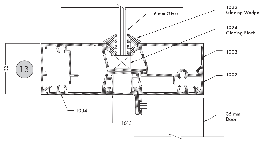
Typical Vertical Section
